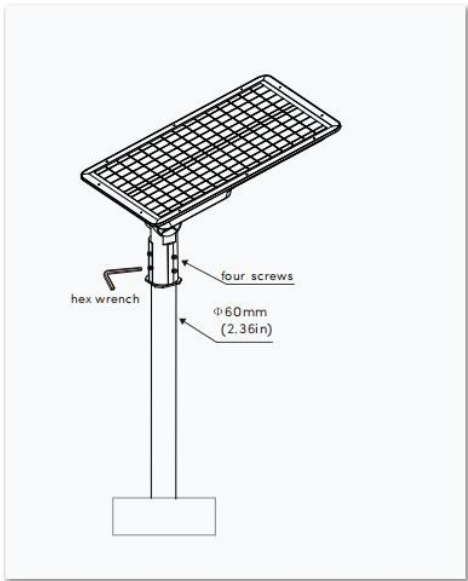
1.Round pole Mounting
