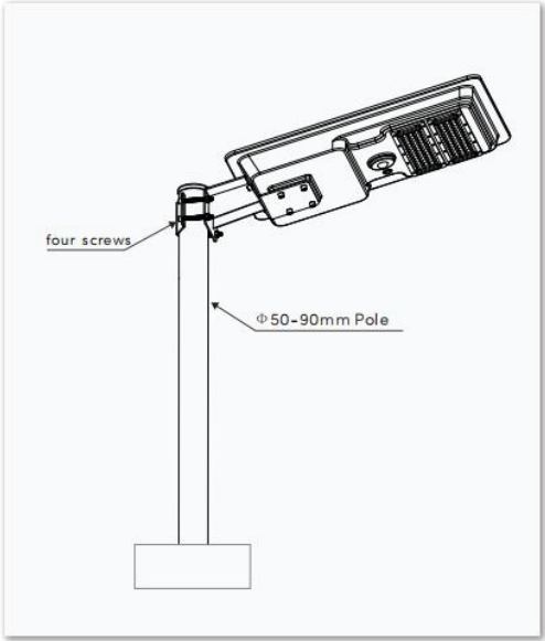
2.Bracket Mounting
